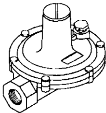
Model 325-5 Port Size: 3/4" x 3/4" MPT Vent Size: 3/8" MPT
