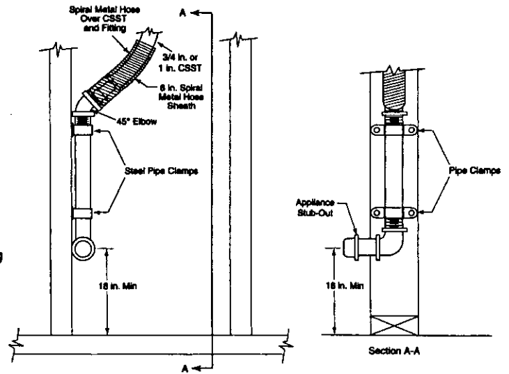
FIGURE 4-38 Appliance termination/stub-out
