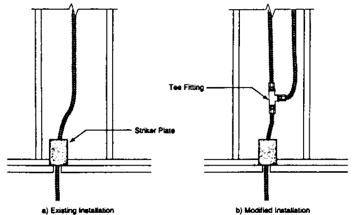
FIGURE 4-39 Extension of existing tubing run
