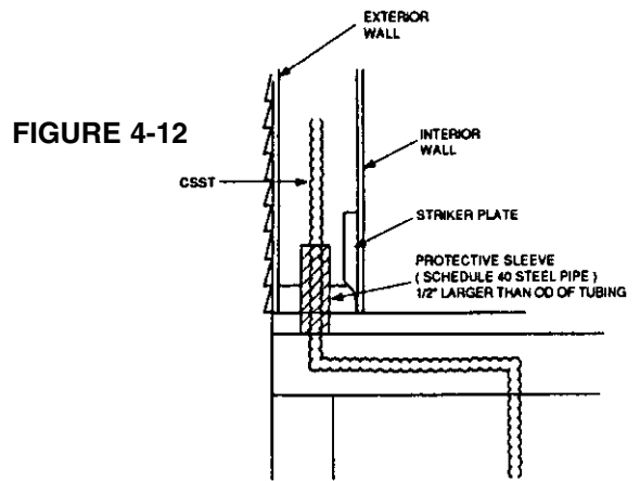
Where Finished Exterior Wall Does Not Permit Installation of Striker Plate, Protective Sleeve is Required.
