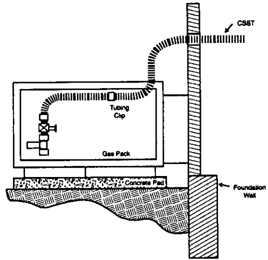
FIGURE 4-35 Pad mounted gas appliance
